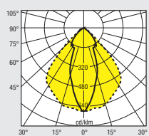
HALODIUM II BT 400W D
