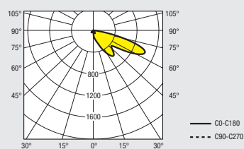
SATURNO II ASM 65° 400 W HQI®-T/NAV®-T
