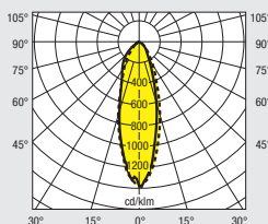
SATURNO II C 2000 W HQI®-TS/DS 20°
