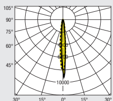
SATURNO II C 2000 W HQI®-TS/DS 8°
