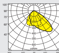
HALODIUM II TS 1500W NDL/NAV AS
