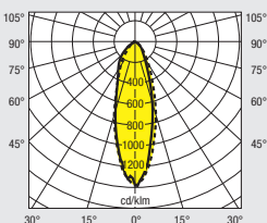
SATURNO II C 2000 W HQI®-TS/DS 30°
