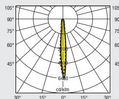
SATURNO II C 2000 W HQI®-TS/DS 10°
