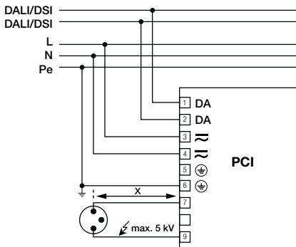
Circuit diagram PCIS class 1 application
