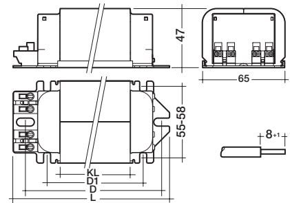
push terminal 0.5–1.5 mm 2
