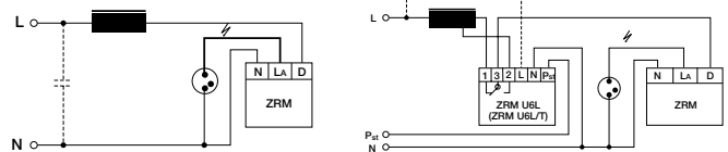
power tapping
