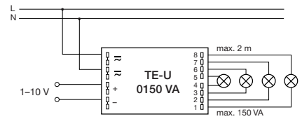
control by external 1–10 V signal
